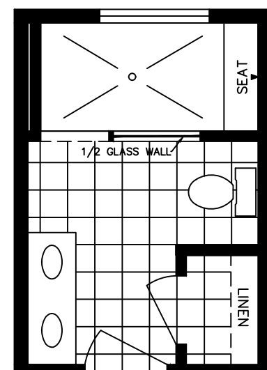
OPT#2 MASTER BATH
