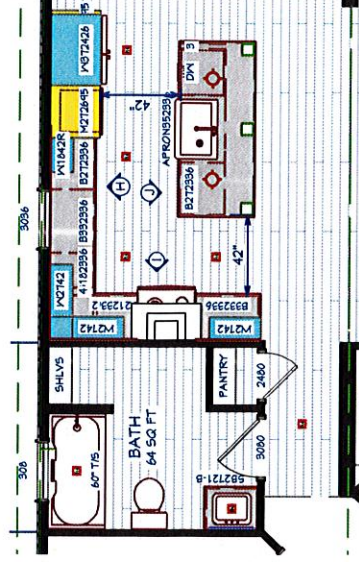
OPTIONAL KITCHEN #1
