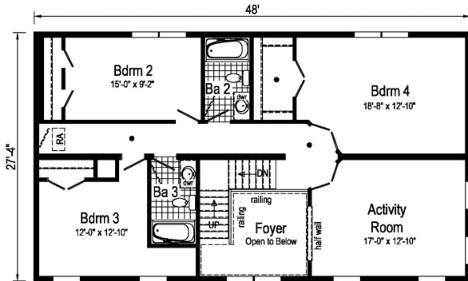
4S3007-R Approx. 3116 Sq. Ft. ● = Std. can light
